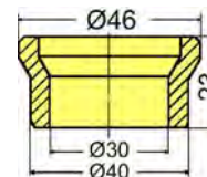
Reduceerhuls 40/30 10505 315 00 00
