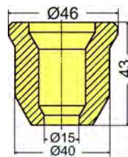
Reduceerhuls IV/I 10505 314 00 00
