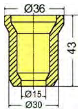
Reduceerhuls 30/15 10505 313 00 00
