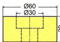
Reduceerinzet 60/30 10506 062 00 00
